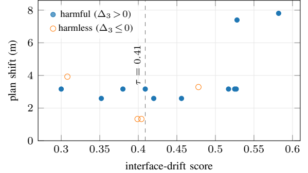
Fig. 6: Interface drift vs. plan shift over the 15 updates (Spearman \approx 0.41 ); dashed line is the balanced threshold.
